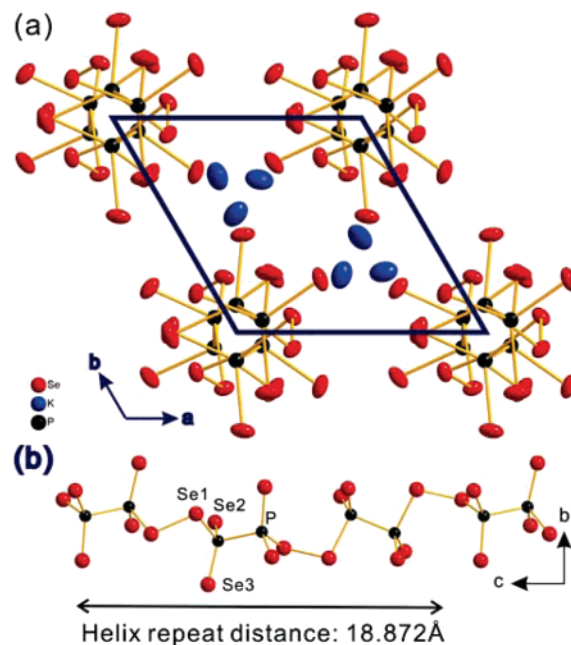
Figure 1. Structure of \text{K}_2\text{P}_2\text{Se}_6 at 298(2) K. (a) The unit cell viewed down the c -axis. The thermal ellipsoids with 30% probability are shown. (b) View of a [\text{P}_2\text{Se}_6]^{2-} chain looking down the a -axis. A helix forms by three [\text{P}_2\text{Se}_6] units and repeats itself at every 18.872 Å.
