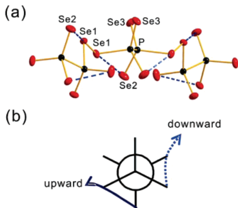
Figure 2. (a) Projection view of a {}^1_2[\text{P}_2\text{Se}_6]^{2-} chain slightly slanted in order to show the staggered anti -conformation of [\text{P}_2\text{Se}_6] . The role of short Se...Se nonbonding interactions (dashed line) along a helix segment is shown. Se(1)...Se(2), 3.559(1) Å. (b) Projection through P–P bonding showing the relationship between short Se...Se nonbonding interaction and chain propagation.
