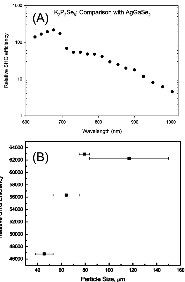
Figure 11. (a) SHG response of K_2P_2Se_6 relative to AgGaSe_2 over a wide range of wavelengths. (b) Particle size to SHG intensities diagram of crystalline K_2P_2Se_6 showing type-I phase-matching.
