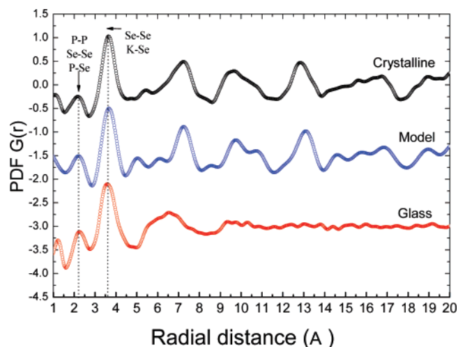
Figure 9. Pair distribution function G(r) of the crystalline and glassy \text{K}_2\text{P}_2\text{Se}_6 .
